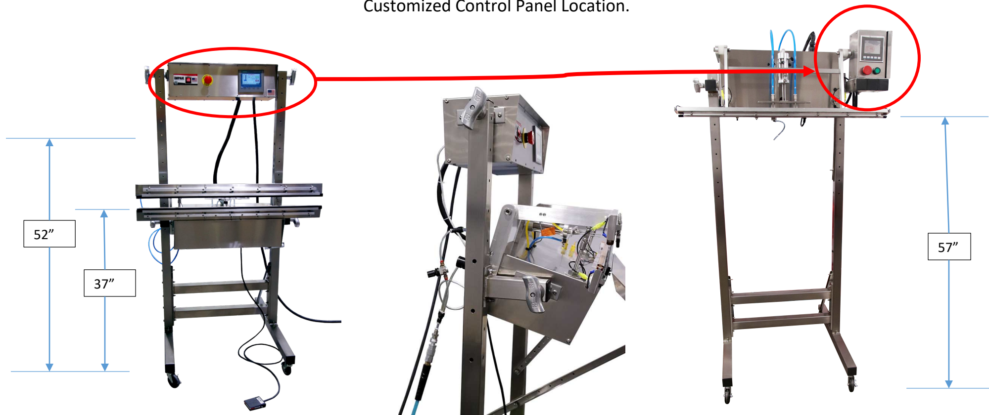
Standard CustomPak Configuration (Top mount controls shown)
